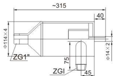
TKF1-17 旋风除尘器 TKF1-17 Whirlwind dust-remover
