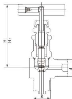
TKJ-2D J24 型外螺纹角式截止阀 TKJ-2D J24 Male and Angle Pattern Stop Valve
