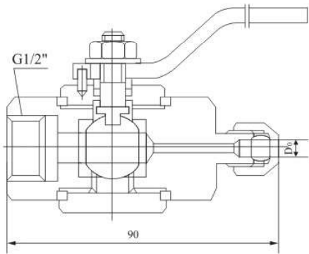
TK9-4 QG.QY1 型气源球阀 TK9-4 QG.QY1 Gas Suply Ball Valve
