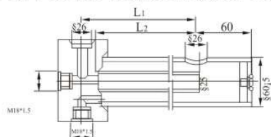
TKF1-15 双室平衡容器 TKF1-15 Two chamber balance vessel
