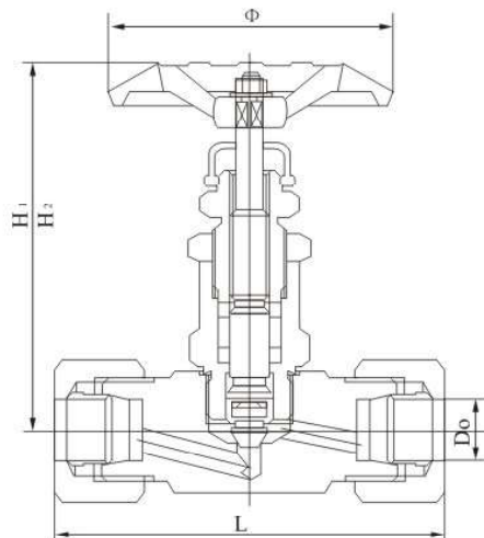
TKJ-1B J91 Collet-type Stop Valve
