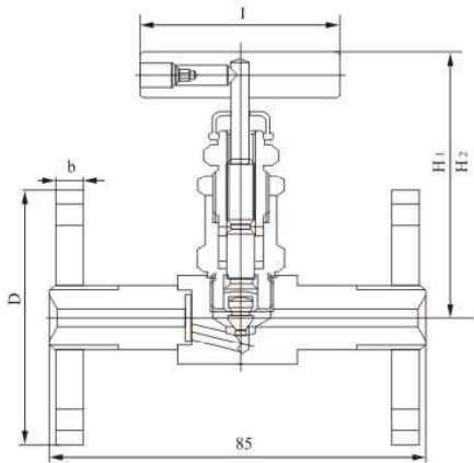
TKJ-11A J41 型法兰截止阀 TKJ-11A J41 Flange-type stop Valve
