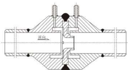
A ISA1932 喷嘴 A ISA1932 nozzle
