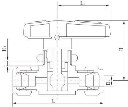
TKQ-4 Q91SA-64 型卡套球阀 TKQ-4 Q91SA-64 Collet Valve
