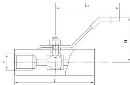
TKQ-2C Q11F-64 型内螺纹球阀 TKQ-2C Q11F-64 Female Screw Ball Valve
