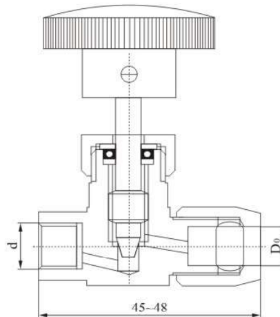
TK6-4 QJ-3A Pneumatic Tube Stop Valve
