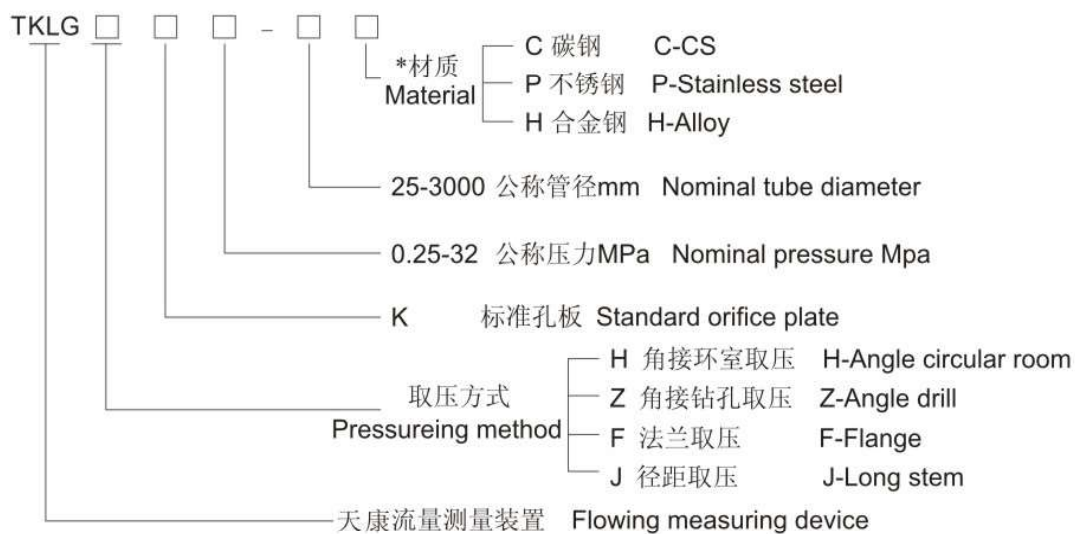
大型孔板 Large Orifice Plate
