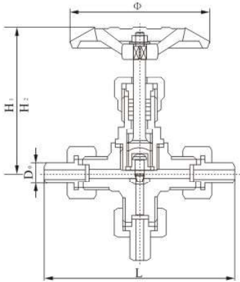
TKJ12-19 J26 W H 型三通截止阀 TKJ12-19 J26 W H 3-way Stop Valve
