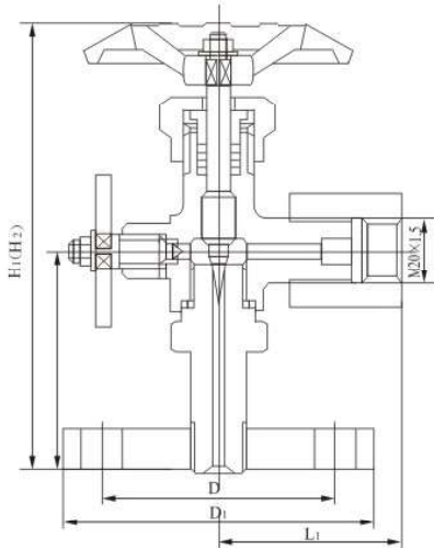
TKJ-10B J49 型压力计用截止阀 TKJ-10B J49 Pressure Gauge Stop Valve
