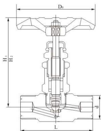
TKJ-2C J21 W 型外螺纹截止阀 TKJ-2C J21 W Male Screw Stop Valve
