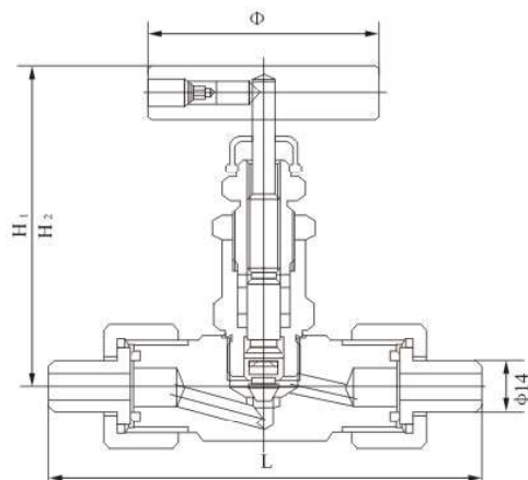
TKJ-2A J21 W 型外螺纹截止阀 TKJ-2A J21 W Male Screw Stop Valve
