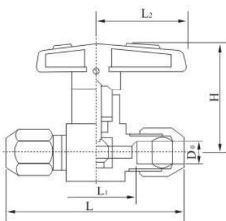
TKQ-7 PQ81SA-64 型排气球阀 TKQ-7 PQ81SA-64 Exhaust Ball Valve
