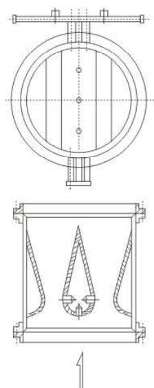
机翼式测风装置 (圆形管道) Measuring wind device in airfoil (in round tube)
