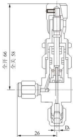
TK12-34 J94H 微型角式截止阀 TK12-34 J94H Miniature angle patten stop valve
