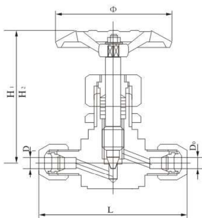
TKJ-1C J91 Collet-type Stop Valve
