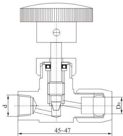
TK6-5 QJ-3B 型气动管路截止阀 TK6-5 QJ-3B Pneumatic Tube Stop Valve
