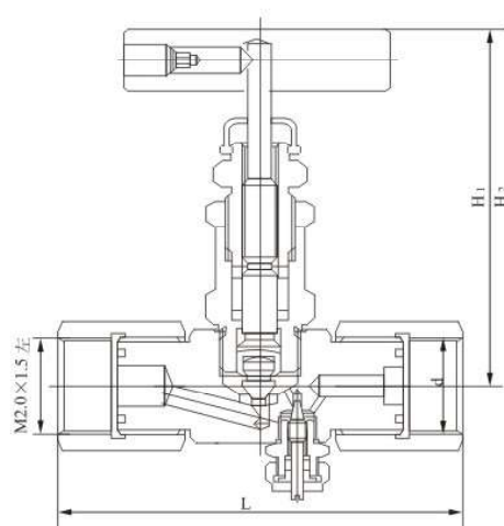
TKJ-6 J11 型节流截止阀 TKJ-6 J11 Throttle Stop Valve
