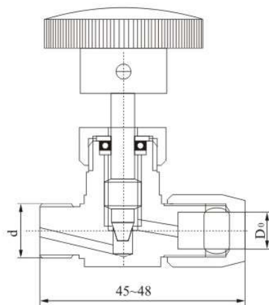
TK6-3 QJ-2A Pneumatic Tube Stop Valve
