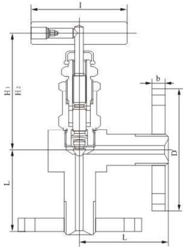
TKJ-11A J44 型法兰截止阀 TKJ-11A J44 Flange-type stop Valve
