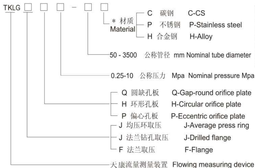
环形孔板 Circular orifice plate
