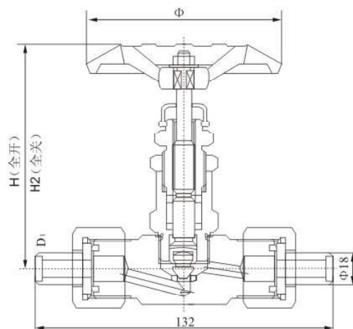
TKJ-2B J21 W 型外螺纹截止阀 TKJ-2B J21 W Male Screw Stop Valve
