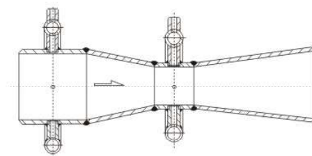
经典文丘里管 Tranditional Wenqiuli Nozzle
