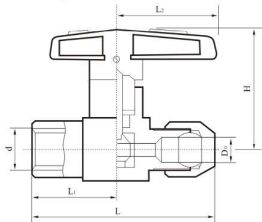
TKQ-1C Q \frac{1}{8} SA-64 型卡箍式球阀 TKQ-1C Q \frac{1}{8} SA-64 Taggle Fype Ball
