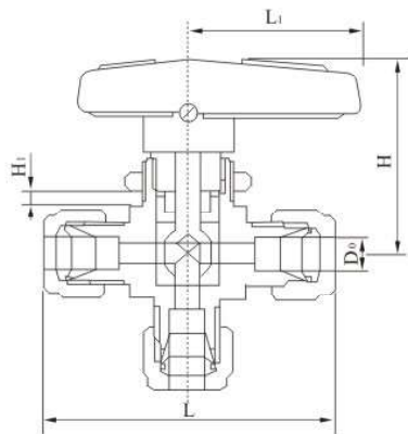
TKQ-6A Q94SA-64 型卡套三通球阀 TKQ-6A Q94SA-64 Collet 3-Way Ball Valve
