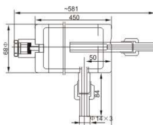
TKF1-25 沉降器(CJ II型液用) TKF1-25 Subside(use for liquid)
