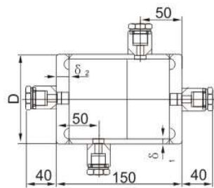
TKF1-14 FG4B 型隔离容器(六) TKF1-14 FG4B Isolation vessel
