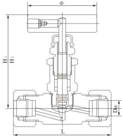
TKJ-1A J91 Collet-type Stop Valve
