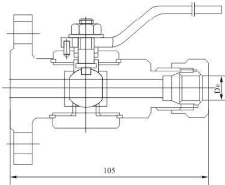
TK9-2 QG.AY1 型取压球阀 TK9-2 QG.AY1 Pressure-taking Ball Valve
