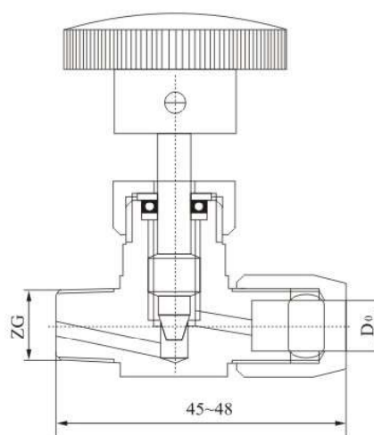
TK6-2 QJ-2A Pneumatic Tube Stop Valve
