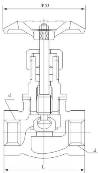
TKJ-3C J11W-16T 型内螺纹铜制截止阀 TKJ-3C J11W-16T Female copper Stop Valve
