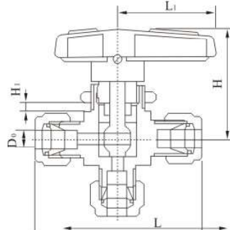
TKQ-8A YFP-1A 型两位一通双卡套球阀 TKQ-8A YFP-1A 2-Direction and 1-Way Double Collet Ball Valve
