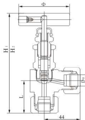
TKJ-1D J94 Collet-type Angle Patten Stop Valve
