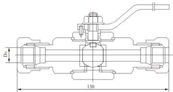
TK9-1 QG.Y1 型卡套式球阀 TK9-1 QG.Y1 Collet-type Ball Valve
