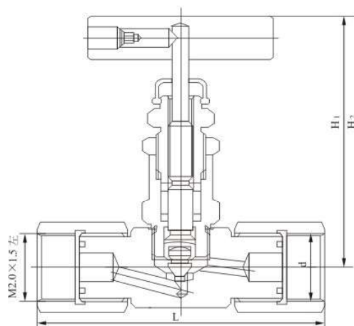
TKJ-5 J11 型压力表截止阀 TKJ-5 J11 Pressure Gauge Stop Valve
