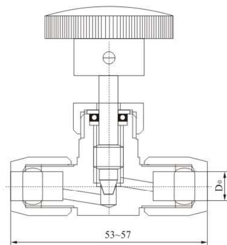
TK6-1 QJ-1 Pneumatic Tube Stop Valve
