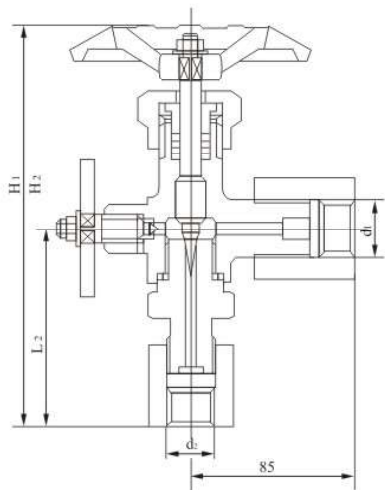
TKJ-10A J29 型压力计用截止阀 TKJ-10A J29 Pressure Gauge Stop Valve
