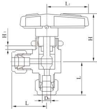
TKQ-5A Q93SA-64 型双卡套角式球阀 TKQ-5A Q93SA-64 Double-Collet Angle Pattera Ball Valve
