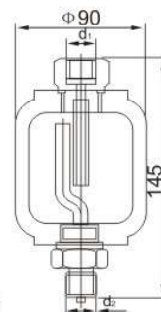
TKF1-19 虹吸管圈 TKF1-19 lphon vessel
